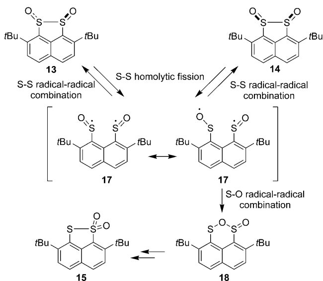
Scheme 3. Formation and reactions of bis(sulfinyl)radical 17 .
